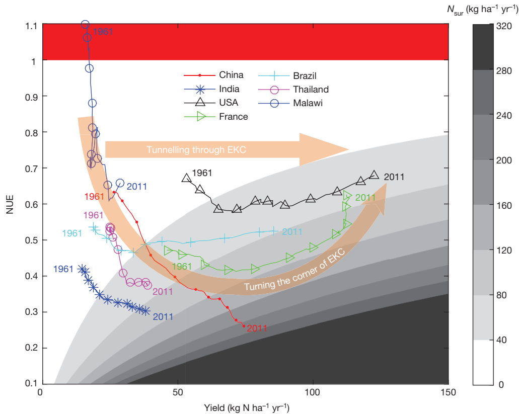
Figure 5 | Historical trends of N_{\text{yield}} , NUE and N_{\text{sur}} for a sample of countries examined in this study. The greyscale shows the level of N_{\text{sur}} . The area covered in red indicates negative N_{\text{sur}} , where the crop production is mining soil N. The data have been smoothed by ten years to limit the impact of year-to-year variation in weather conditions. Curves moving
