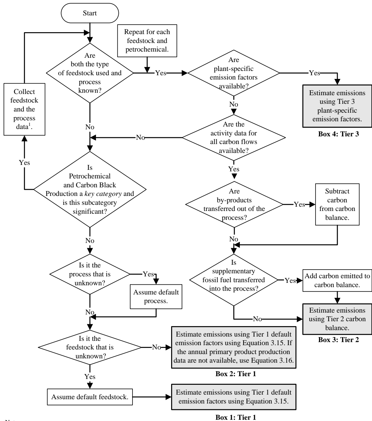
Figure 3.8 Decision tree for estimation of CO 2 emissions from petrochemical industry and carbon black industry
