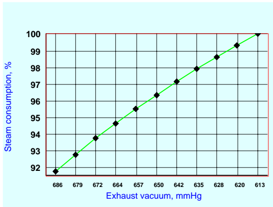
Fig 6a : Effect of exhaust vacuum on steam consumption in condensing type turbine
